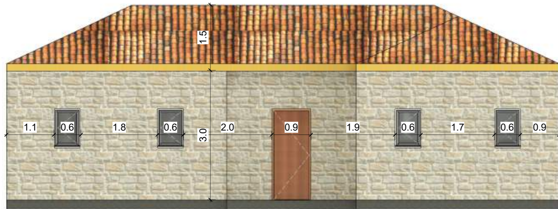
PRRJA 1-1
