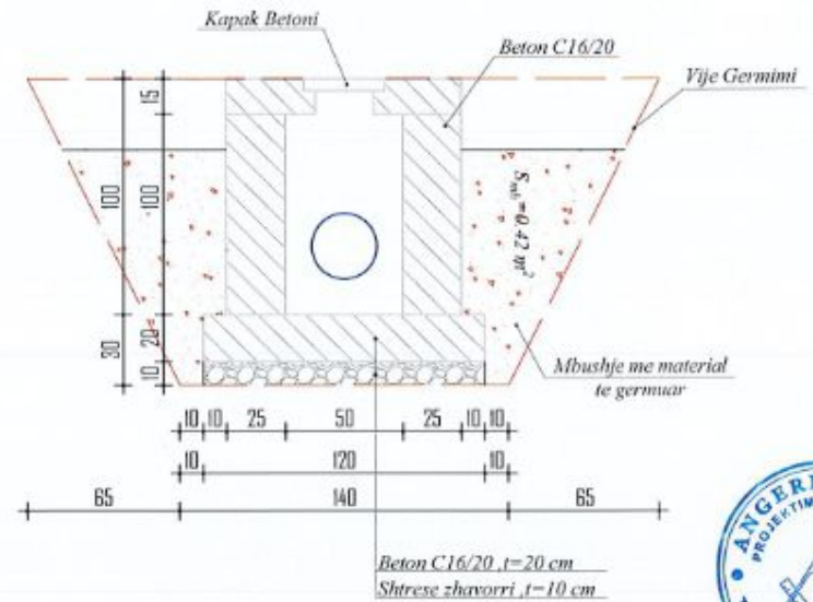
PRERJA B-B SH. 1:25
