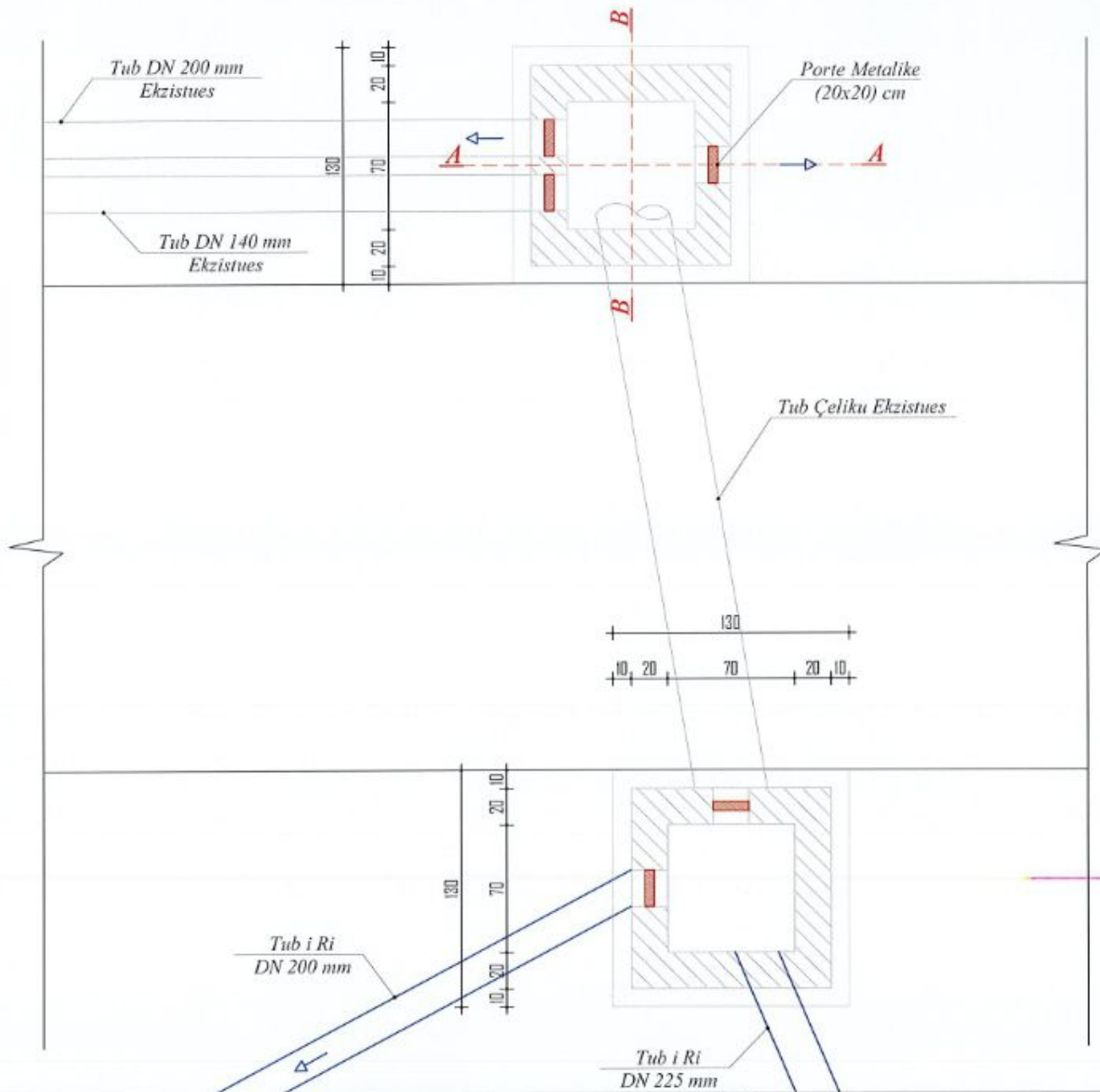
PLANIMETRIA SH. 1:25
