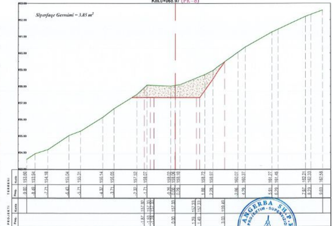
Km.0+068.97 (PK-8)
