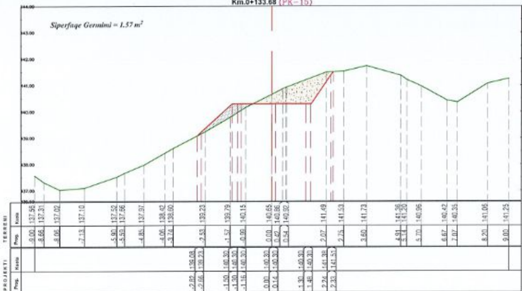
Km.0+133.68 (PK-15)
