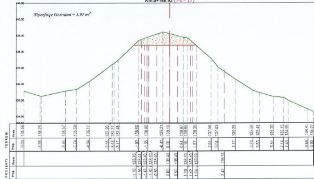
Km.0+146.92 (PK-17)
