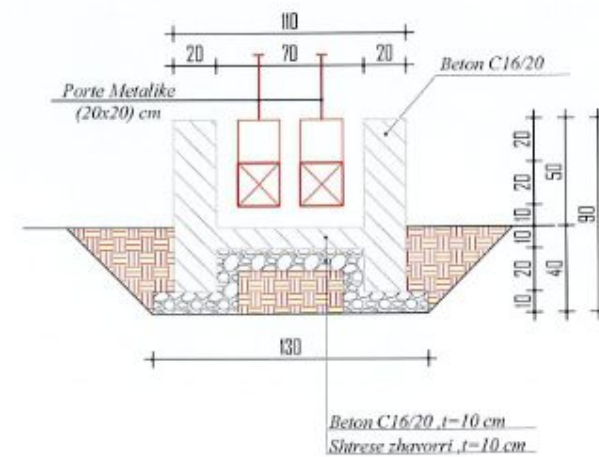
PRERJA B-B SH. 1:25
