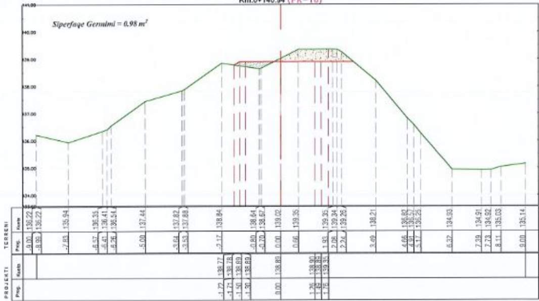
Km.0+140.94 (PK-16)
