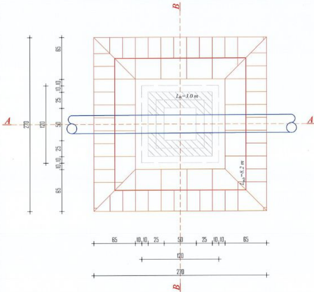
PLANIMETRIA SH. 1:25
