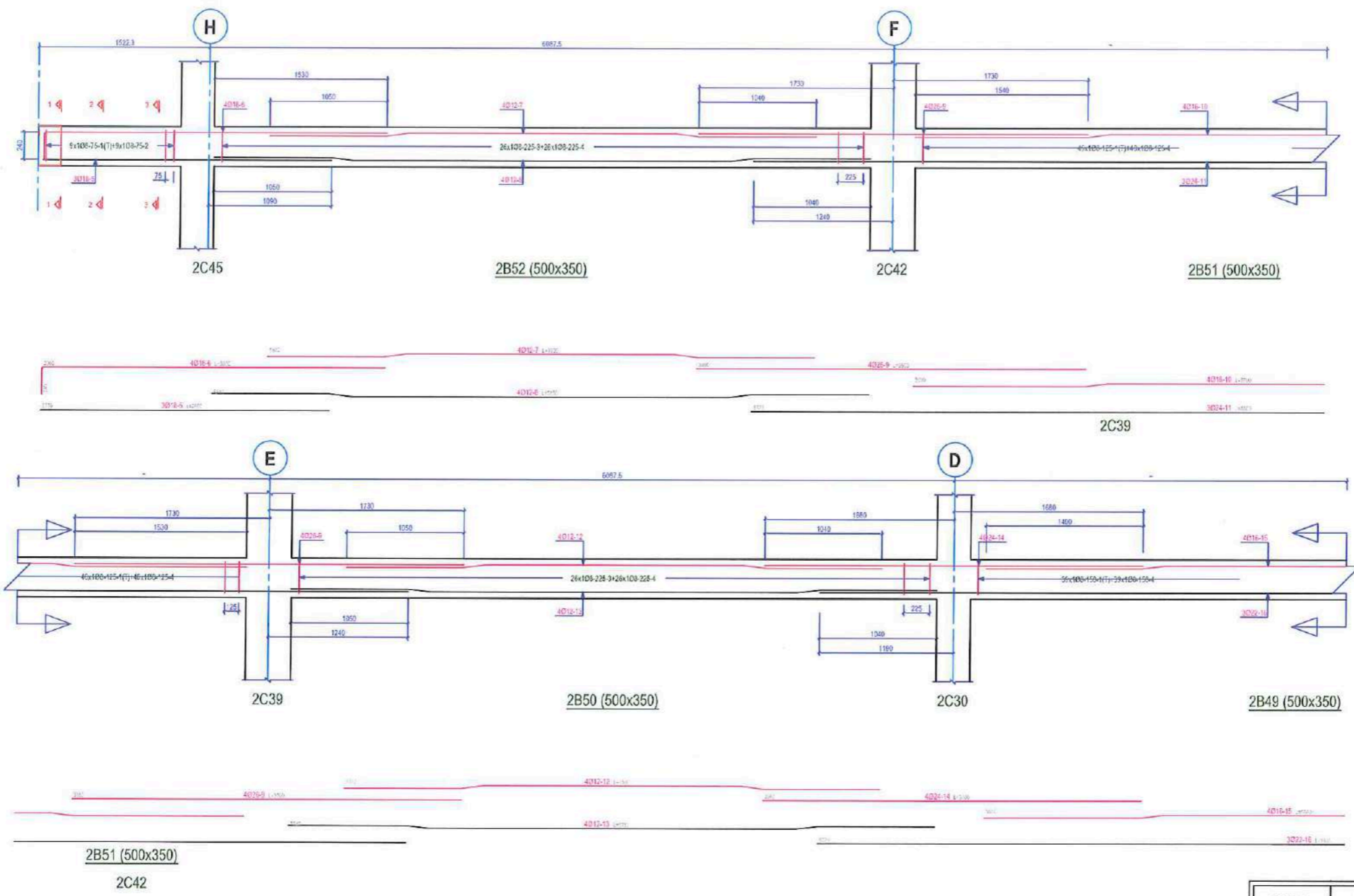
BEAM ELEVATIONS1
