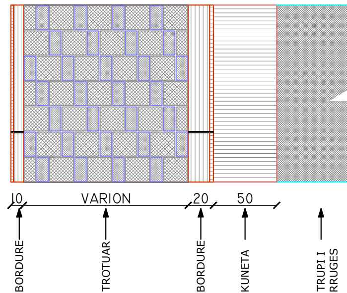
PLAN PLANIMETRIA
