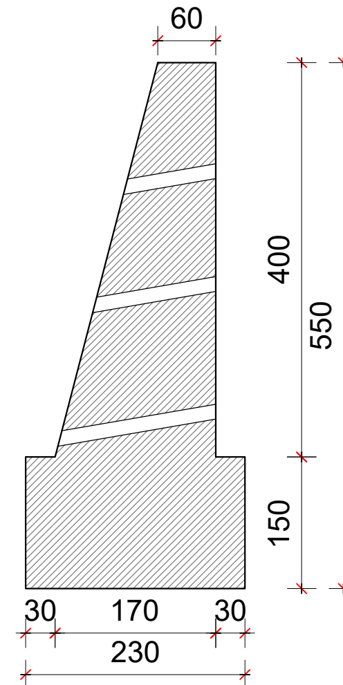
MURE BETONI H=4.0m
