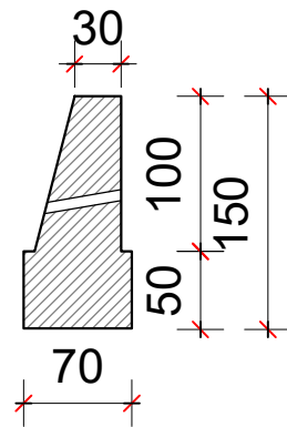
MURE BETONI H=2.7m
