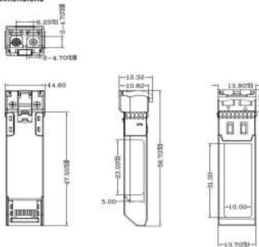
Mechanical Dimensions
