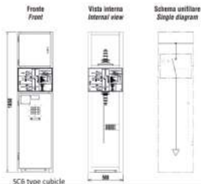
SC6 type cubicle
