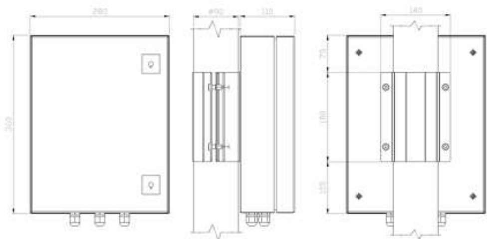
Version with Band-it pole brackets
