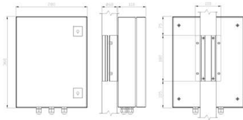
Version with 90 mm pole brackets
