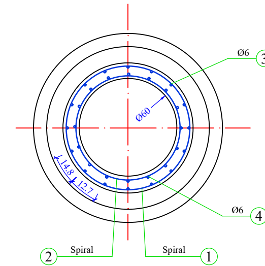
PLAN SH.1:20
