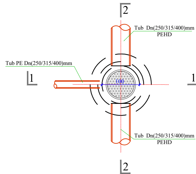
PLAN SH.1:50
