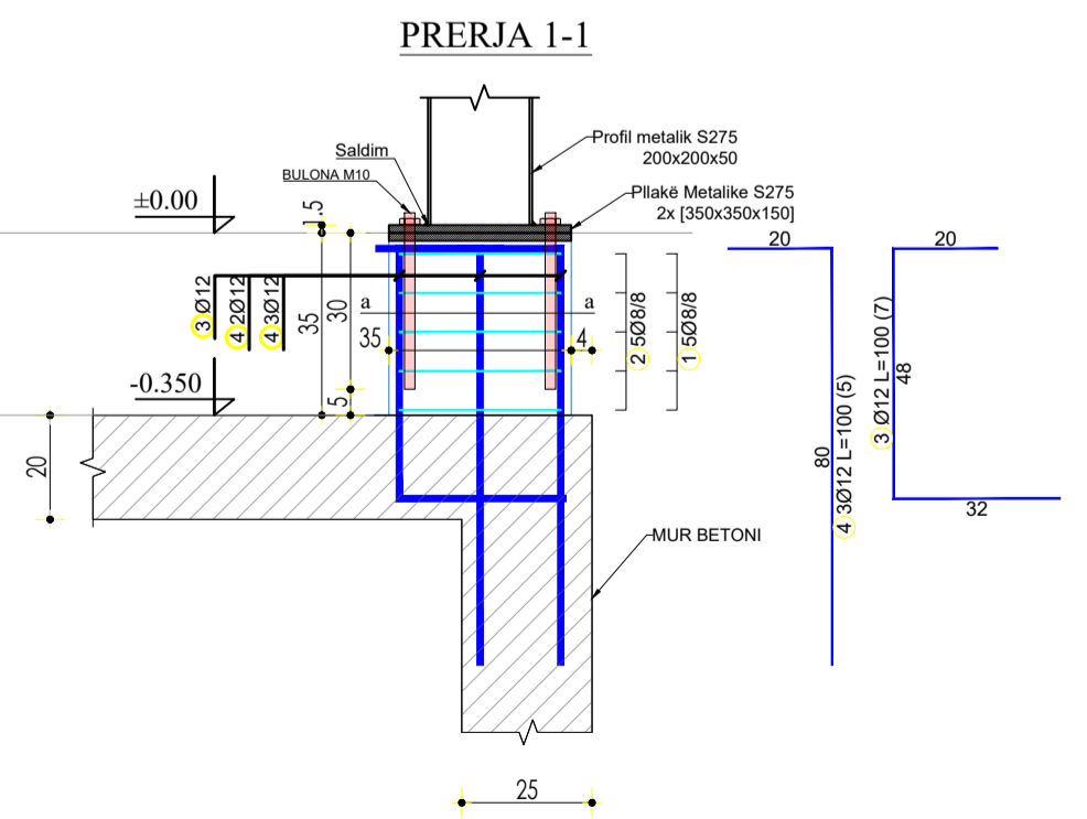
RAST III LIDHJA PROFILIT 200x200x5 MBI MUR BETONI PRERJA 1-1
