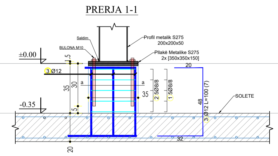
RAST II LIDHJA PROFILIT 200x200x5 MBI SOLETE PRERJA 1-1
