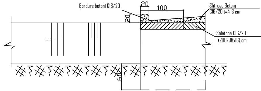
PRERJA 1 - 1 SH. 1:50
