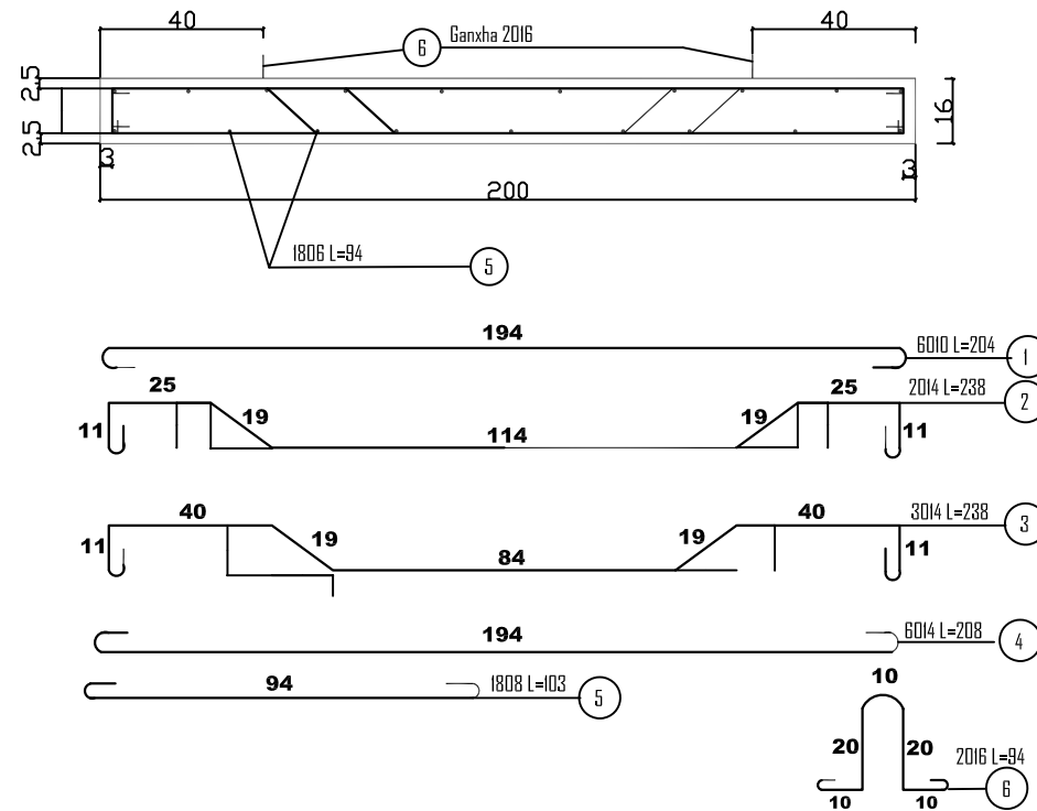
ARMIMI I SOLETONIT SH. 1:20
