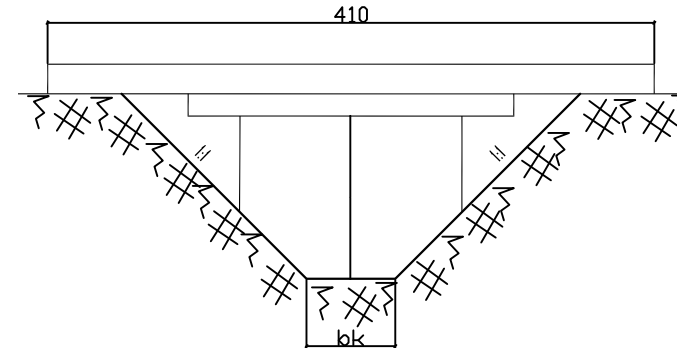
PRERJA 2 - 2 SH. 1:50
