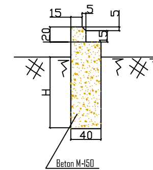
PRERJA a - a SH. 1:50
