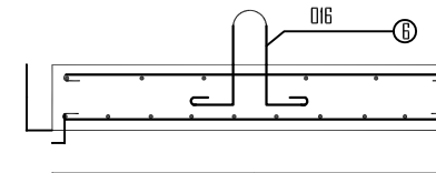
PRERJE TERTHORE SH. 1:20
