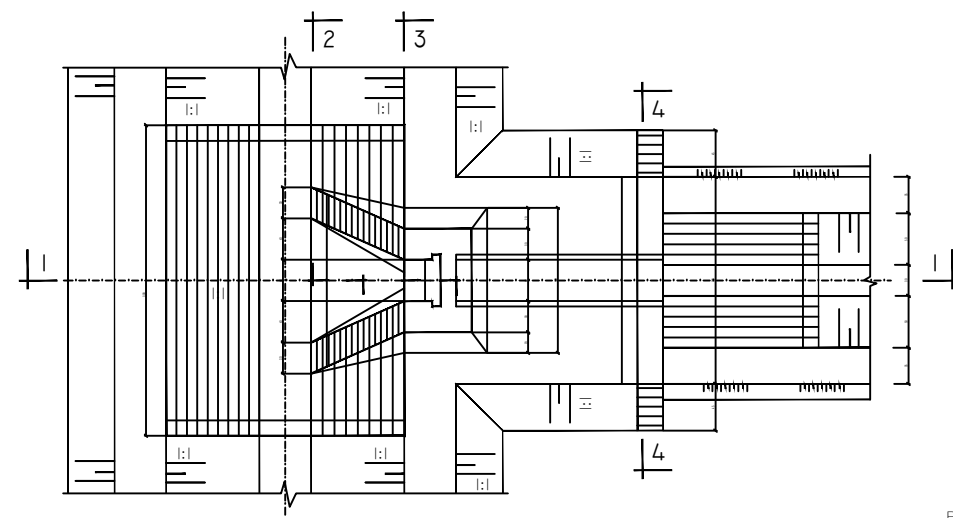
PLANIMETRIA SH. 1:50
