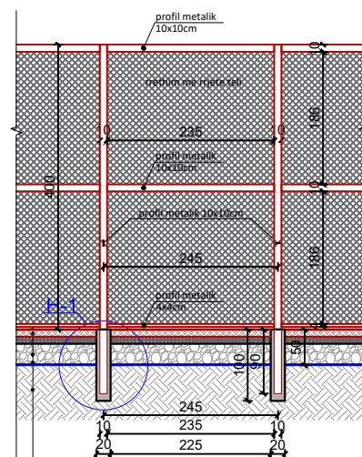
DETAJI 1 - RRETHIMI I FUSHES
